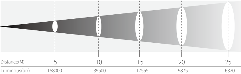
Beam Angle: 3.3°
